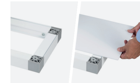
Thanks to the new design, the modular system can be mounted quickly and easily.
